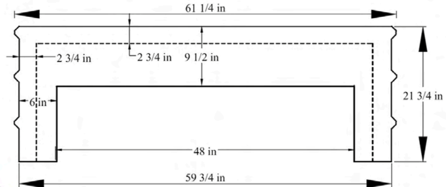
REAR ELEVATION
