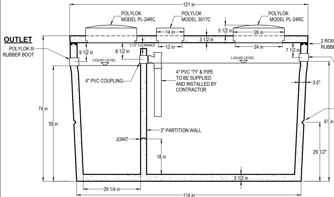
SIDE ELEVATION - SECTION A-A
