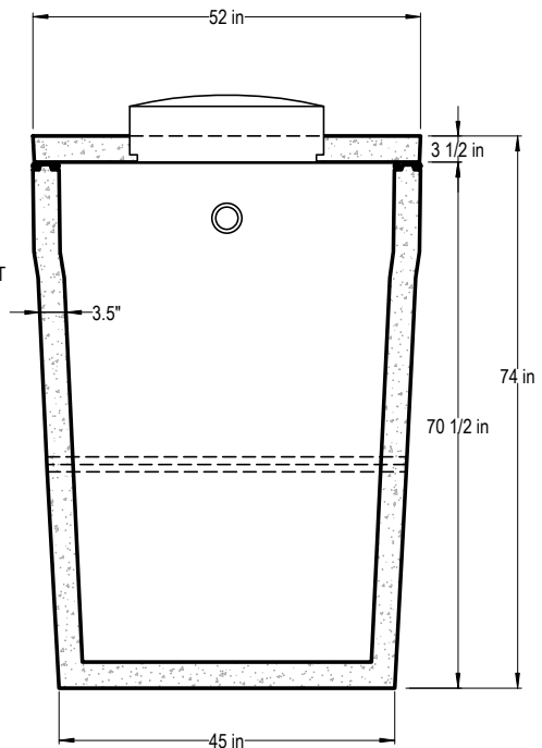
END ELEVATION SECTION B-B
