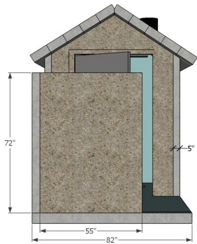
FRONT
